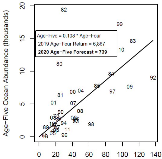
FIGURE II-3. Regression estimators for Klamath River fall Chinook ocean abundance (September 1) based on that year's river return of same cohort. Numbers in plots denote brood years.
