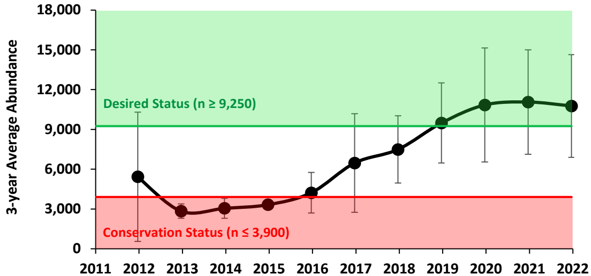
Figure 1. Three-year running average estimated abundance of White Sturgeon \geq 167 cm FL from the lower Columbia River, 2012–2022. Less than three years of data were available prior to 2012 so averages are not available. Error bars represent one standard deviation.
