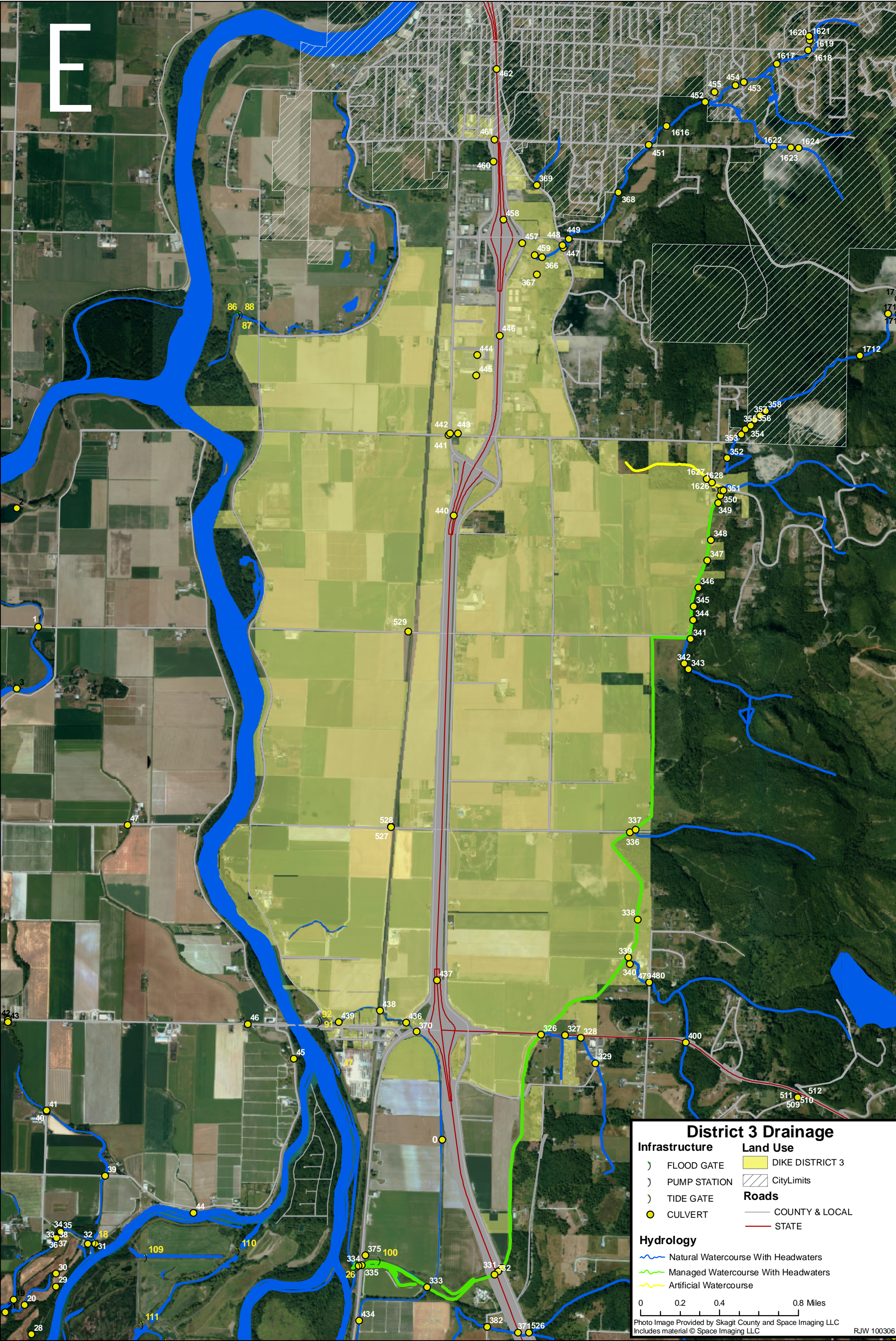
Figure 2: Skagit County Dike District #3, watercourse classifications and drainage infrastructure.
