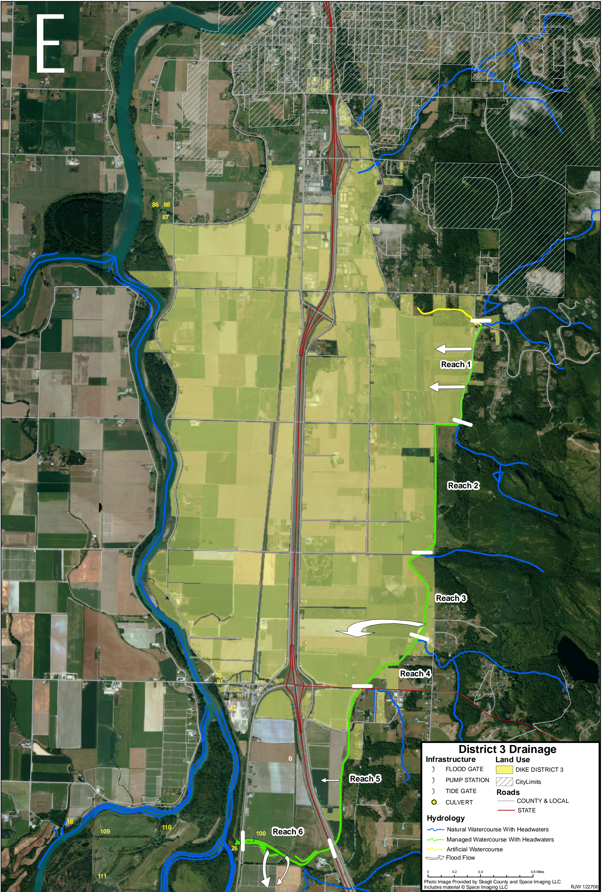
Figure 2a: Skagit County Dike District #3, Flood Flow Management Strategy.
