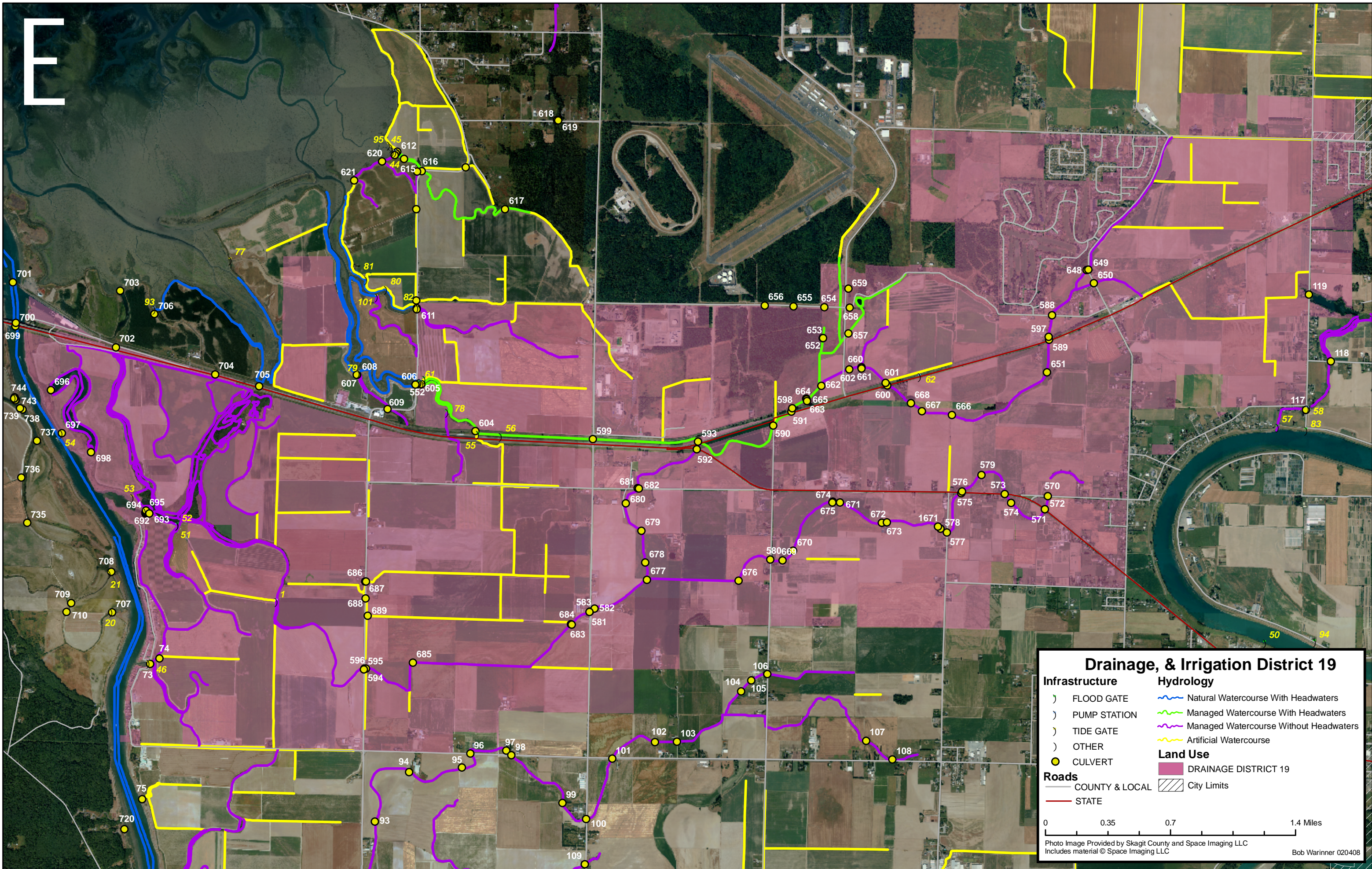
Figure 2: Skagit County Dike, Drainage, and Irrigation District #19, watercourse classifications and drainage infrastructure.
