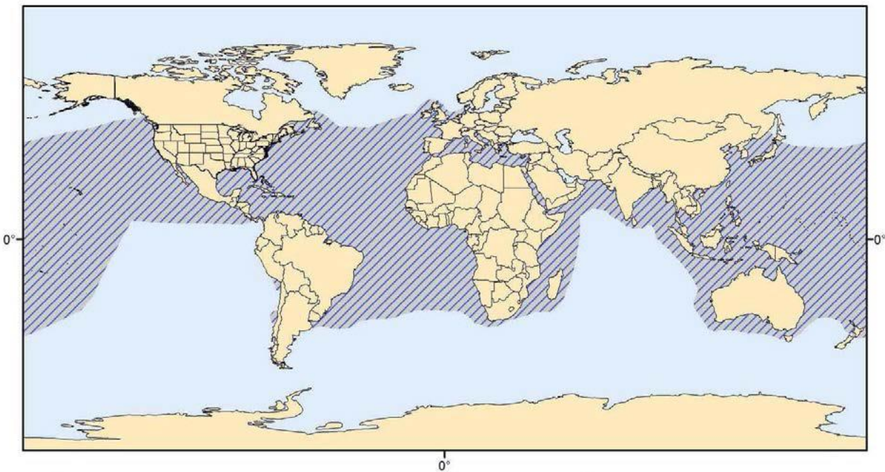
Figure 1. Loggerhead sea turtle global distribution
