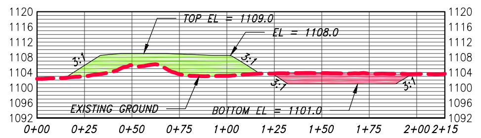
3 ISLAND 5 7 SECTION
