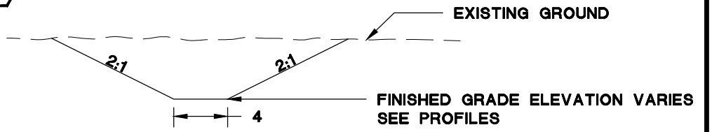
3 SWALE 1 11 TYPICAL
