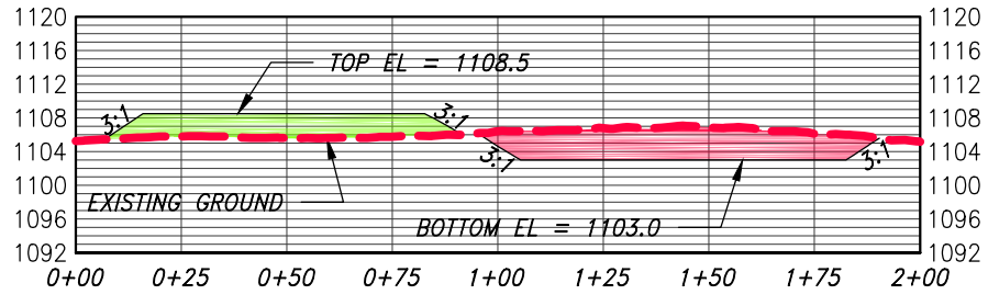
2 ISLAND 4 7 SECTION
