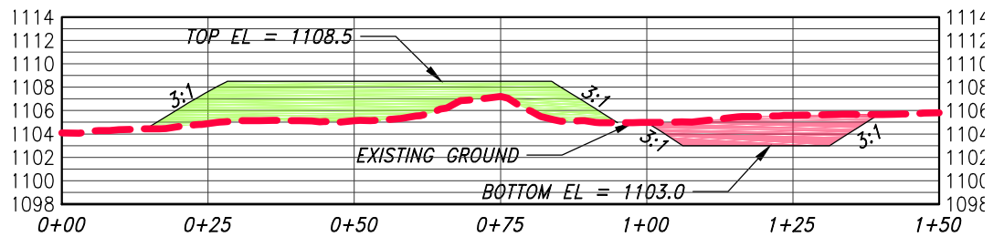
2 ISLAND 3 6 SECTION
