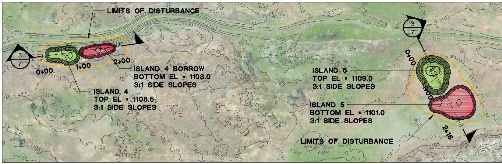
1 ISLANDS 4 & 5 7 PLAN VIEW
