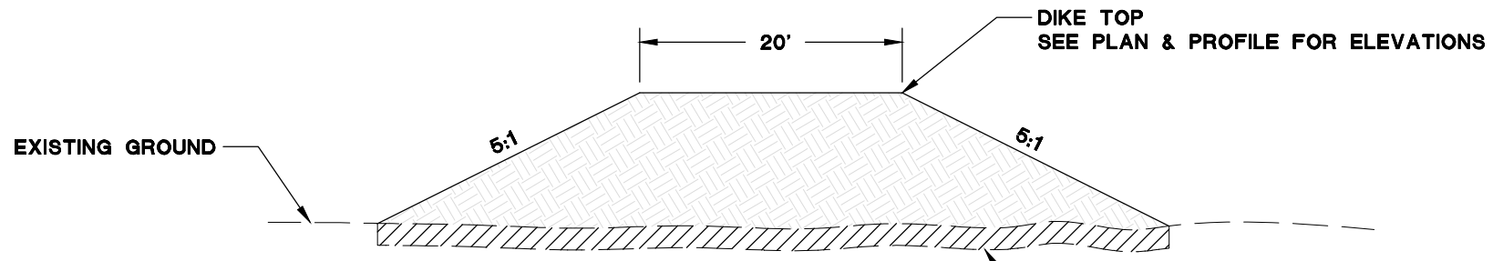
2 DIKE DETAIL 13 TYPICAL N.T.S. STRIP ORGANICS A MINIMUM OF 6" OR PER THE SPECIFICATIONS
