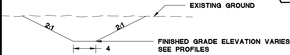
2 NEW INLET DITCH 11 TYPICAL
