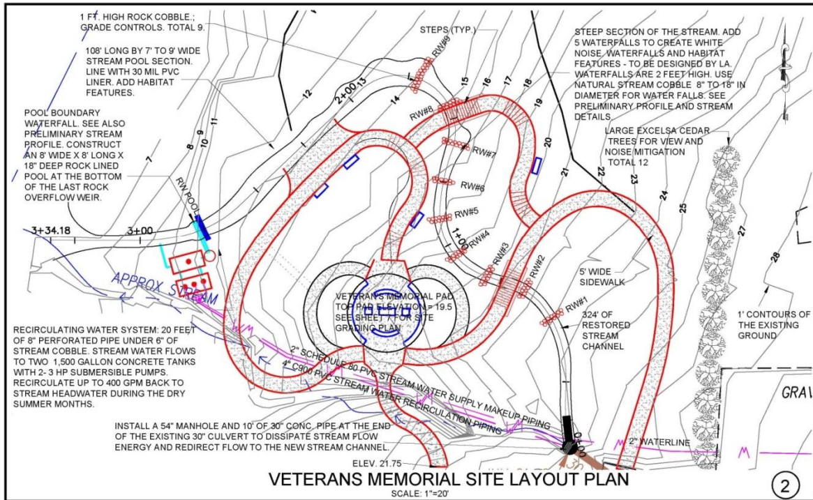
FIGURE 2: Proposed Development Site Plan
