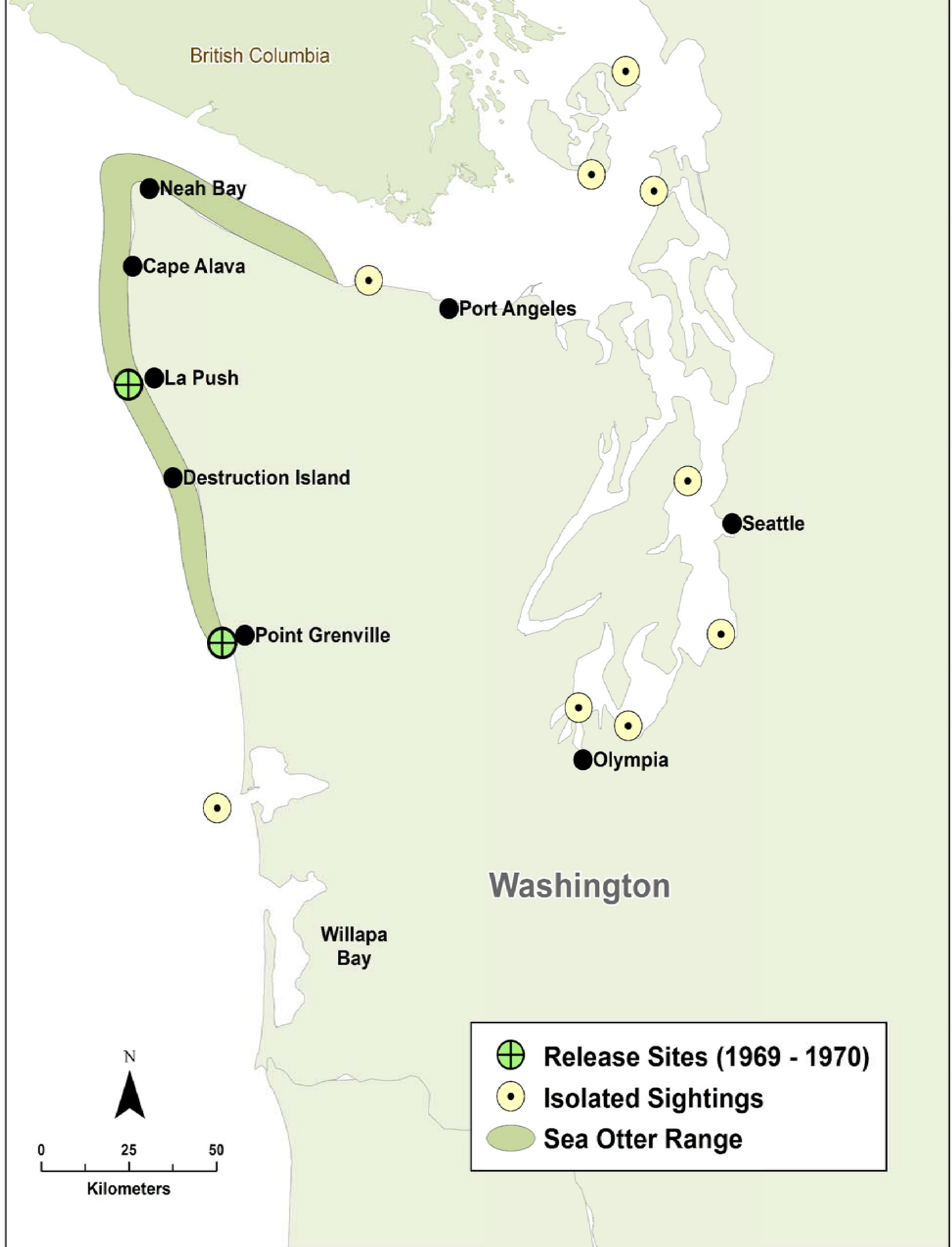
Figure 3b. Approximate current distribution of the sea otter in Washington, 1969 to 1970 release sites and isolated sightings in Washington (adapted from Lance et al
